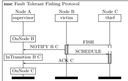
Figure 6: Supervised work-stealing in the absence of faults
