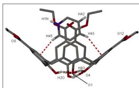
Fig. 2. Selectively labelled asymmetric unit in the single crystal X-ray structure of [\text{PyH}][\text{3-H}] . Hydrogen bonding interactions are shown as split-colour dashed lines and CH... \pi interactions are shown as red dashed lines. Hydrogen atoms (apart from those involved in hydrogen bonding and CH... \pi interactions) omitted for clarity.
