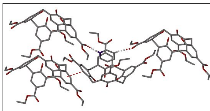
Fig. 2. Selectively labelled asymmetric unit in the single crystal X-ray structure of [\text{PyH}][\text{3-H}] . Hydrogen bonding interactions are shown as split-colour dashed lines and CH... \pi interactions are shown as red dashed lines. Hydrogen atoms (apart from those involved in hydrogen bonding and CH... \pi interactions) omitted for clarity.
