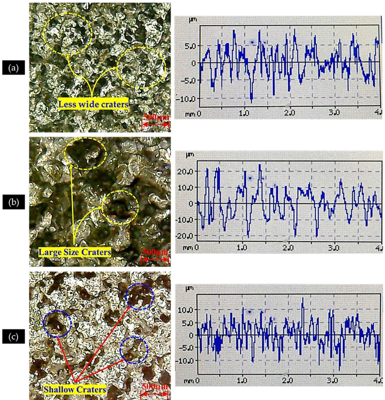
Fig. 5 Micrograph's comparison of electrodes with their graphical demonstration. (a) Al is giving less wide craters with low peak-to-valley distance. (b) Br is showing poor surface finish with large size craters and
