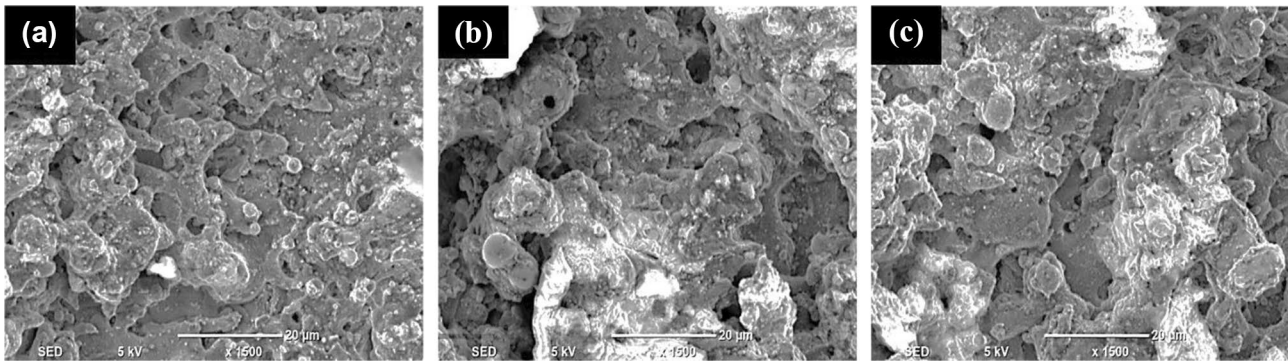
Fig. 6 SEM images of machined surface using electrode of (a) Al, (b) brass, and (c) Cu
