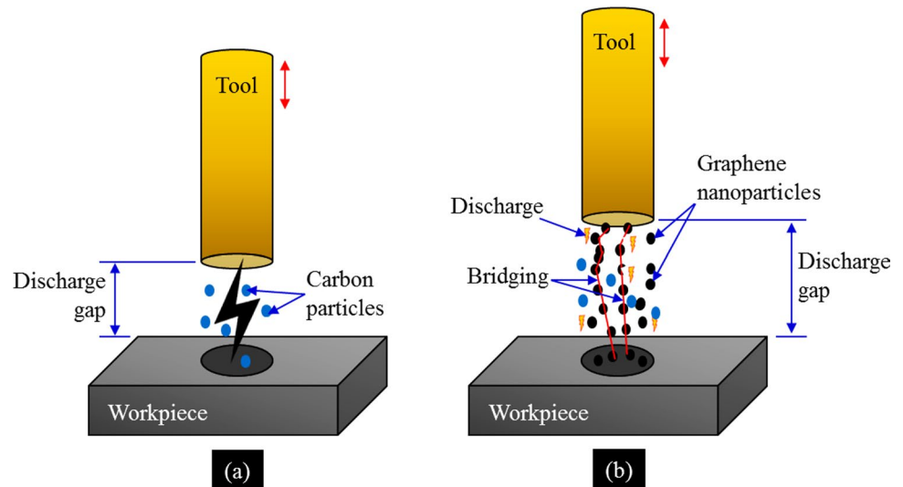
Fig. 13 Schematic illustrates the role of nanopowder in EDM dielectric. (a) Kerosene-based EDM. (b) Graphene nanoparticles mixed EDM
