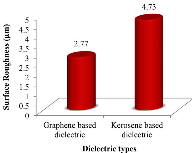
Fig. 14 Comparative analysis of SR under graphene and kerosene based dielectrics
