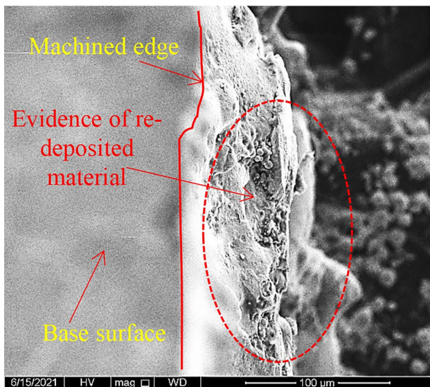
Fig. 10 SEM image showing re-deposited layer on specimen's surface
