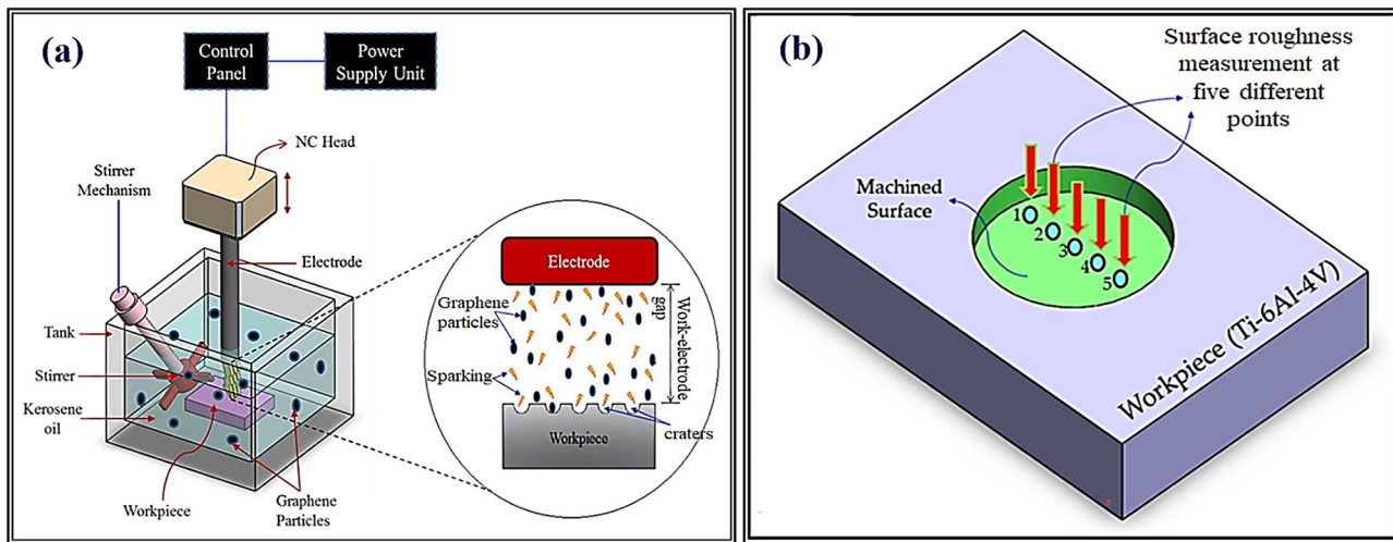
Fig. 1 Experimental arrangement of EDM. (a) Schematic and basic principle of EDM. (b) Schematic for the measurement of SR magnitude at various points
