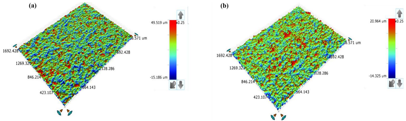
Fig. 11 3D roughness profiles at (a) optimal settings and (b) non-optimal settings
