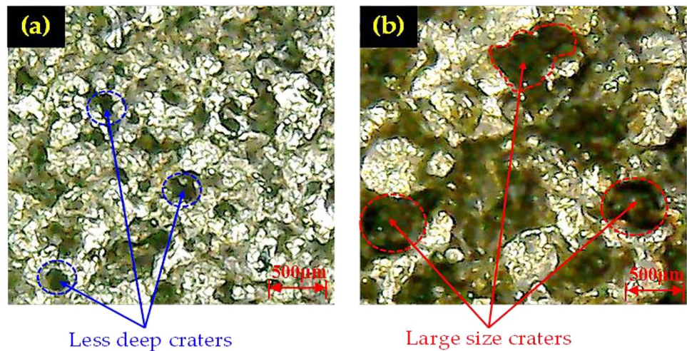
Fig. 4 Micrographs at two different polarities. (a) Positive polarity with small size craters. (b) Negative polarity with large and deep craters
