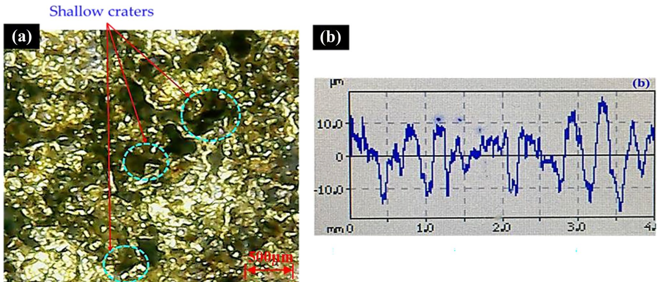
Fig. 8 Effect of DC at 8 amps. (a) Micrographs appearing shallow craters on the workpart surface. (b) Variation in R_a values representing considerable peaks and valleys
