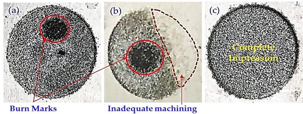
Fig. 2 Preliminary trials’ images of machined specimen indicating (a) burn marks, (b) burn mark with an incomplete machined surface, and (c) complete impression
