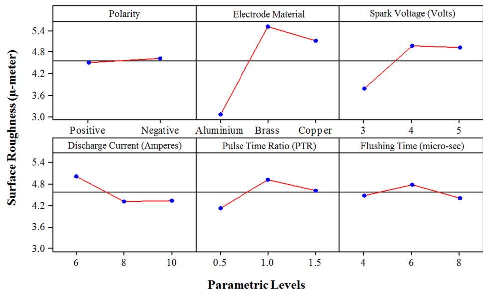
Fig. 3 Parametric Plots against each control variables using graphene nanoparticles in the dielectric medium
