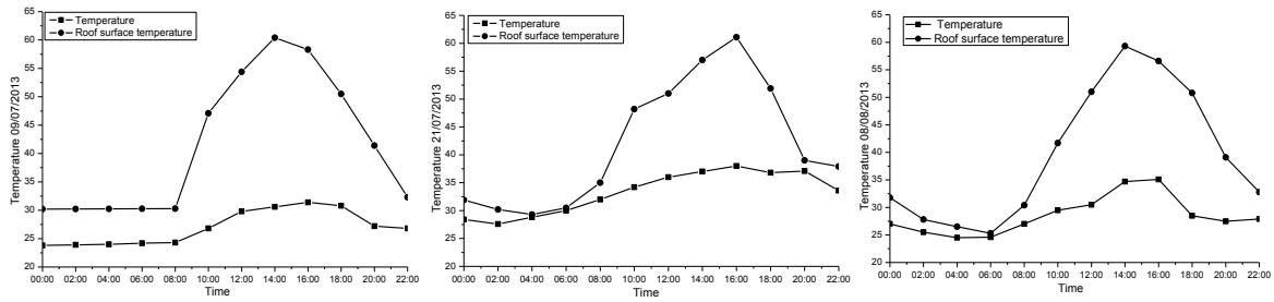
Figure 9 Roof Surface Temperatures on the Three Days.
