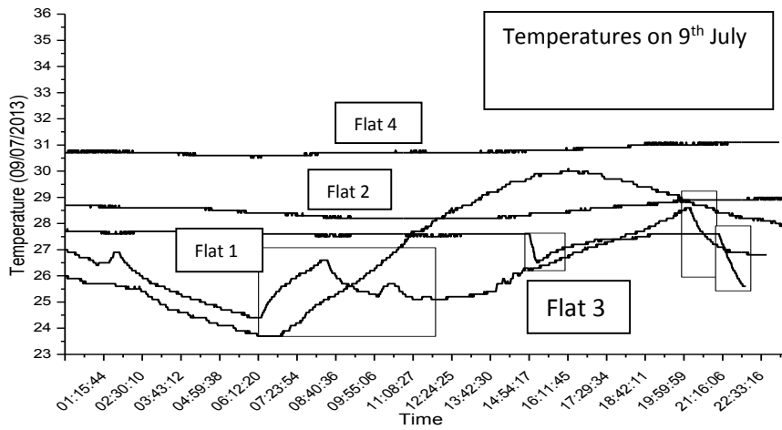
Figure 3 Main room temperatures on the 9 th July
