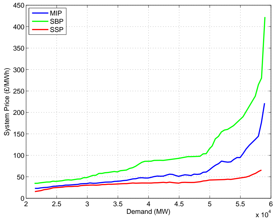
Figure 3: The mean system price profiles of Mean Index Price (MIP), System Buy Price (SBP) and System Sell Price (SSP) versus demand.
