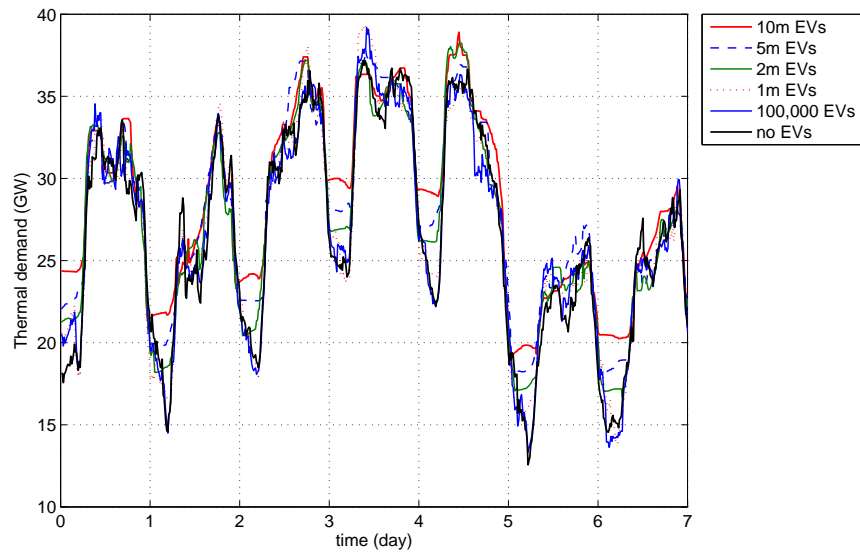
Figure 7: Comparison of load profiles with increasing number of electric vehicles step wise up to 10 million vehicles charging in the network with 14 GW of wind power capacity.
