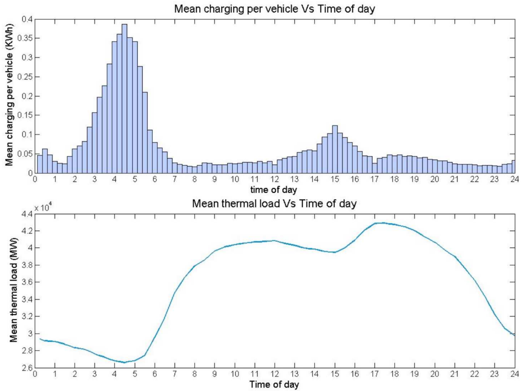
Figure 9: Comparison of the average daily charging distribution for a single vehicle (in 15 minute time bars) versus the average daily load profile with 4.6 GW of network wind power capacity.
