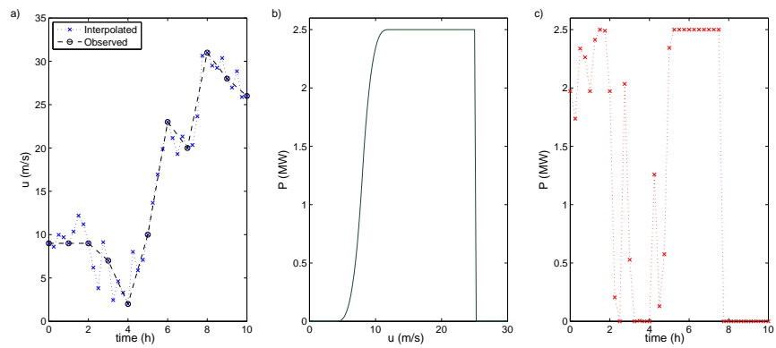
Figure 4: Illustration of calculating wind power generation from hourly wind measurements for a 10-hour section: a) hourly readings, adjusted from 10 m to 100 m as black circles; interpolated values with random perturbations as blue crosses. b) The Nordex N90 performance curve as power output against wind speed. c) The calculated power output at the interpolated times given the interpolated wind speeds and the performance curve.
