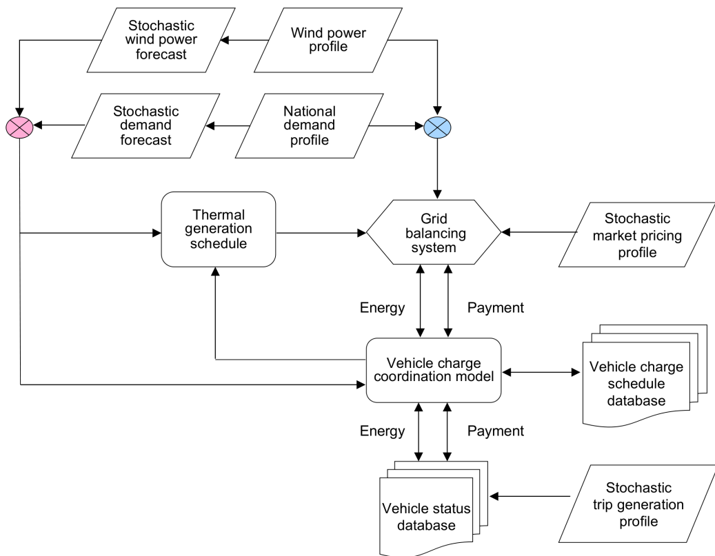
Figure 1: Flow Diagram of the balancing model.
