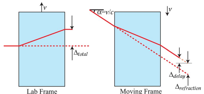
Fig. 1. (Color online) Transverse shift imparted to a light beam by a moving medium can be calculated in the frame of the medium.
