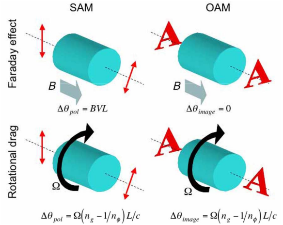
Fig. 2. (Color online) Application of a magnetic field along the axis of the rod leads to a rotation of the transmitted polarization but not of the image. Conversely, the mechanically induced ether drag associated with a rotating cylinder rotates both the polarization and the image through the same angle.
