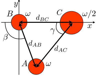
FIG. 1. (Color online) Schematic representation of the system of three harmonic traps with broken spatial symmetry. Traps A and B have a trapping frequency \omega and trap C has a trapping frequency \omega/2 .
