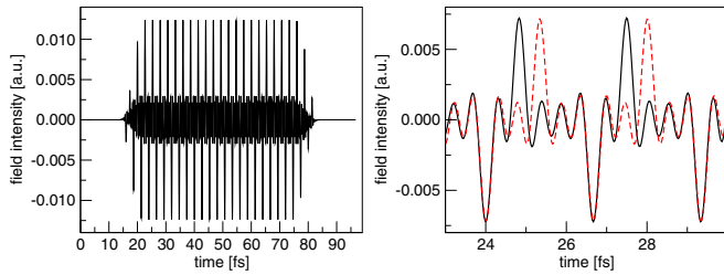
FIG. 2. (Color online) Synthesized subcycle pulse trains. The left panel shows the intensity versus time (in femtoseconds). Only pulse train A is shown because, at this scale, waveform B looks the same. The right panel shows two fundamental periods in both pulse streams. Note that the strong unipolar impulses are the same in amplitude and only differ in their relative timing.
