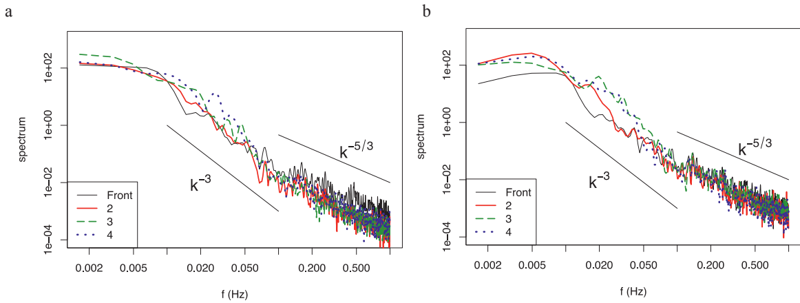
Fig. 5. Spectrum of streamwise velocity at the first four turbines, (a) at a wind direction of 223° when all turbines are fully shaded by the front turbine the front turbine, and (b) at a wind direction of 229° when the second turbine is only partially shaded by the front turbine.
