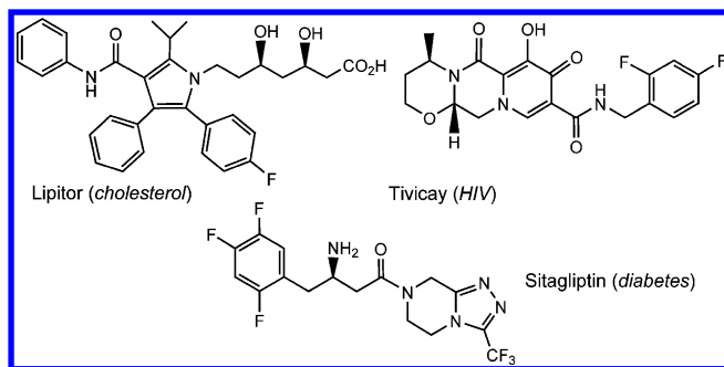
Chart 1. High-Value Fluoroaromatic Compounds
