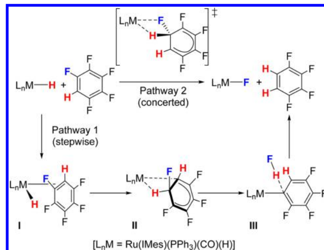
Scheme 2. Mechanisms of Ru-Catalyzed HDF of C_6F_5H to 1,2,3,4- C_6F_4H_2
