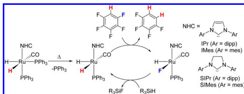
Scheme 1. Ru-Catalyzed HDF of C_6F_5H to 1,2,3,4- C_6F_4H_2
