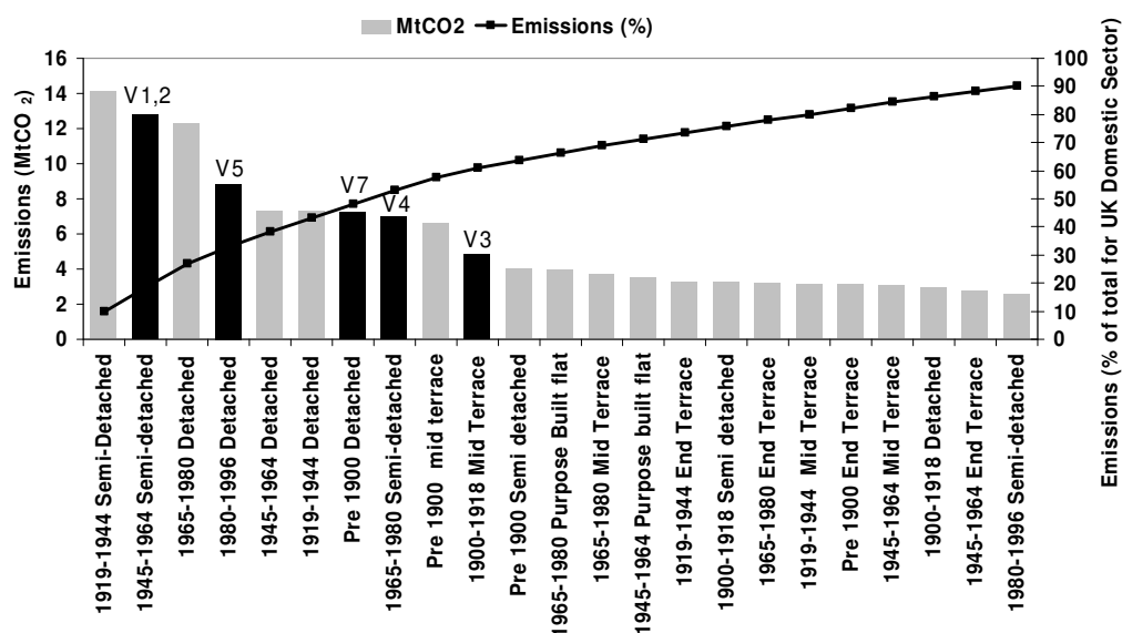
Figure 2: Tarbase Domestic sector variants (pre 1996) – CO 2 emission attribution
