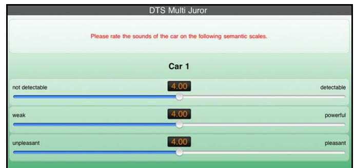
Fig. 5. Evaluation interface.
