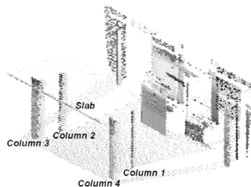
Figure 4: Scanned Point Cloud
