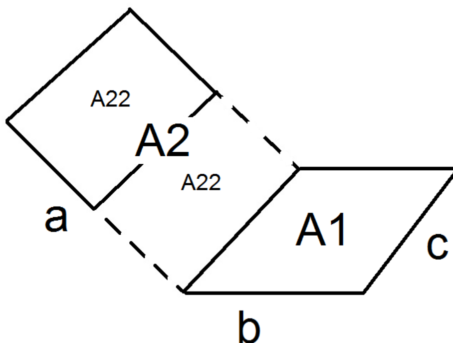
Figure 1. Schematic for the computation of view factor A_{1-22} to be incorporated for radiance from surface 1 to surface 22. Note: surface 1 represents the ground and surface 22 the PV module. A_1 = 1 , F_{1-2} = 0.169 , F_{1-21} = 0.151 , F_{1-22} = F_{1-2} - F_{1-21} = 0.018 .
