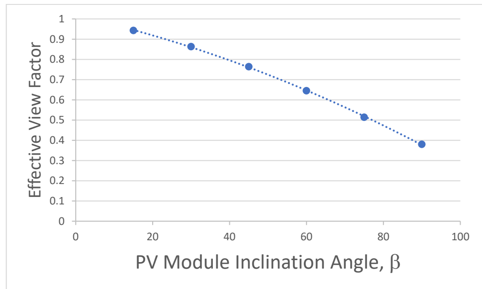
Figure 2. Relationship between the effective view factor and angle of inclination \beta of the PV module. This relationship is valid only for the given geometry.
