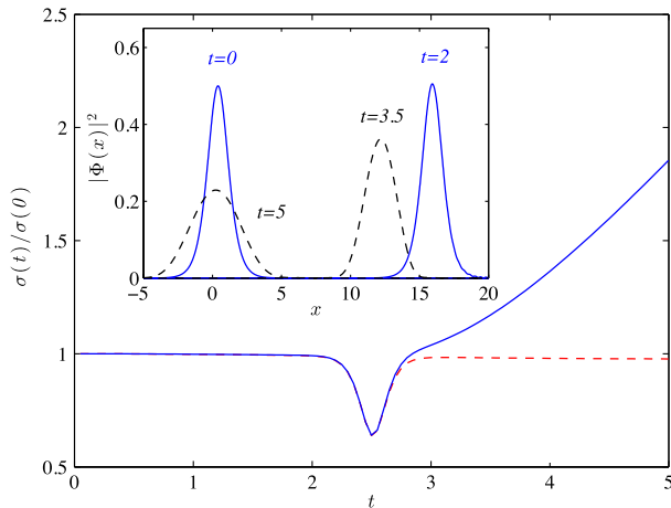
FIG. 2 (color online). The normalized width \sigma(t)/\sigma(0) of the bright soliton. The blue solid line shows \sigma(t)/\sigma(0) with current strength (g_{11} - g_{22})kN/(S_t\hbar\Omega) = 0.125 and (gN/S_t) \times (2m/\hbar^2k) = -0.5 , while the red dashed line indicates the width of an initially identical soliton without the current nonlinearity ( a_1 = 0 ). After reflection the soliton starts expanding due to the change in nonlinear strength. The inset shows snapshots of the density of the soliton prior to (solid blue) and after reflection (dashed black) at times t = 0, 2.0, 3.5 , and 5.0 . All lengths are in units of 1/k and time in units of 2m/\hbar k^2 .
