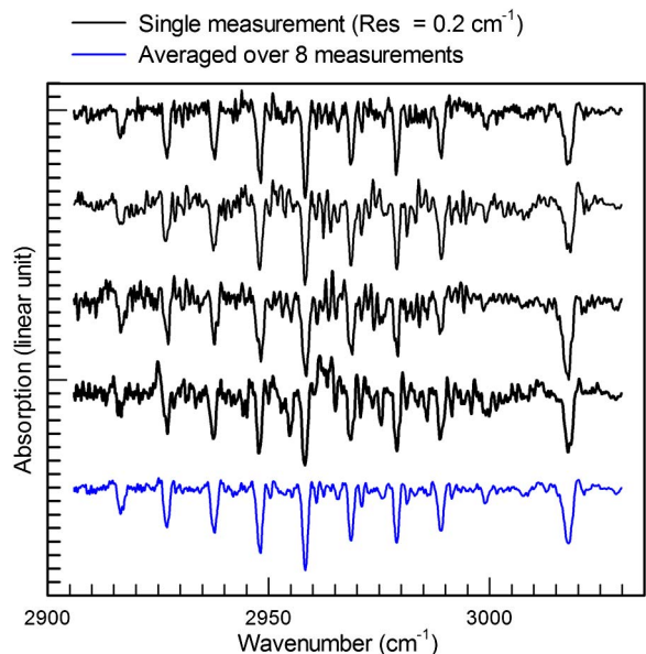
Fig. 4. Normalized methane absorption spectra for single measurements (top 4 traces, black) and an averaged spectrum (bottom trace, blue).
