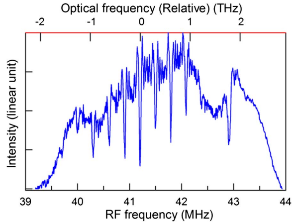
Fig. 3. Fourier-transform spectrum expressed in the RF (lower axis) and optical (upper axis) domains.
