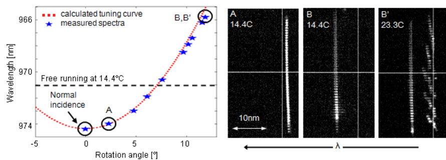
Fig. 5. Wavelength vs. angle of the VHG obtained in the folded cavity configuration and examples of measured spectra. The laser was operated at 20A of drive current. (Note: the non-uniform intensity pattern and a slight tilt of the image are due to aberrations in the imaging system.)
