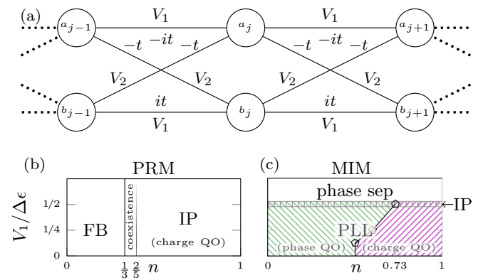
FIG. 1. (a) Creutz ladder with sites a_j and b_j in the j th unit cell with hopping and interaction parameters given by the Hamiltonian Eq. (1). (b) Phase diagram of the purely repulsive model (PRM) with V_1 > 0 and V_2 = 0 as a function of density n . For n \leq 1/3 the physics is captured by the lower flat band (FB) without interactions. For n > 2/5 an itinerant-paired (IP) phase of fermions exists with dominant charge quasiorder (QO). In between we find a coexistence regime. (c) Phase diagram of the mixed interaction model (MIM) with V_1 = -V_2 > 0 with a pair Luttinger liquid (PLL) for V_1/\Delta\epsilon \lesssim 1/2 , with phase (charge) QO for lower (higher) densities marked by three points. Around V_1/\Delta\epsilon \simeq 1/2 an IP with highly enhanced superconducting correlations exists for n \leq 0.73 . Larger interactions give phase separation.
