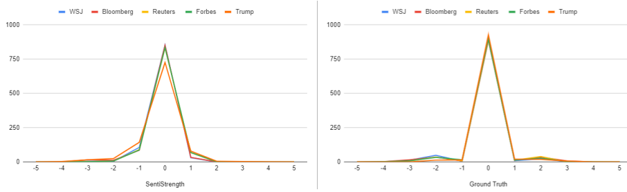
Fig. 1. Distributions of compound SA_c scores as generated by SentiStrength (left) and Ground Truth (right).
