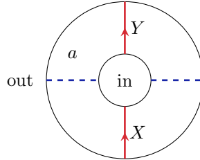
Figure 5: A cylinder of total area a with two parallel defect lines labeled by X, Y \in D_1 . The dashed lines indicate a cell decomposition of this surface.
