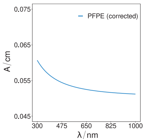
Fig. 5. The determined optical absorbance coefficients of the PFPE sample over the spectral range of 300 nm to 1000 nm, as calculated from the corrected transmissivity intensity.
