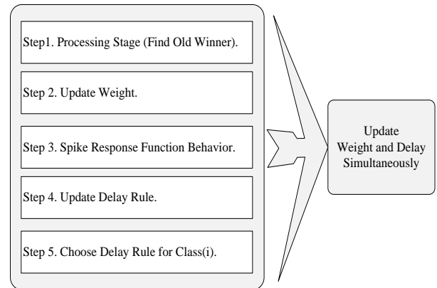
Fig. 2: General site-specific proposed to make SRF stable
