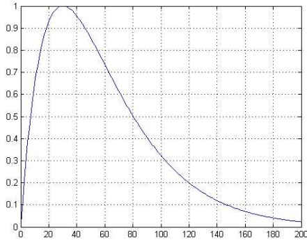
Fig. 1: Spike Response Function
