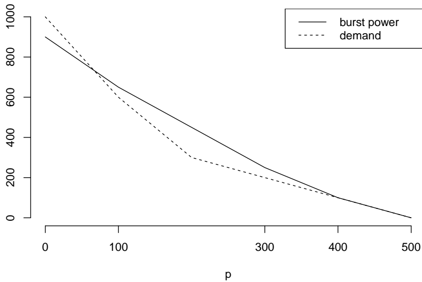
Figure 2: Example 2.1: energy-power transforms e_s^0(p) and e_d^0(p) at time 0 of the burst-power profile (of the initial stored-energy configuration) and of the demand process ( d(t) , t \geq 0 ). The set \pi(0) defined in the proof of Theorem 2.1 is given by \{0, 100, 300, 400, 500\} and is indicated on the horizontal axis. Both e_s^0(p) and e_d^0(p) are convex decreasing functions of p and the function e_s^0(p) is linear between successive points of the set \pi(0) . The value of the expression (2.7) is equal to 100 (the maximum being attained at p = 0 ), which, from Theorem 2.1 is the minimum unserved energy demand over all policies.
