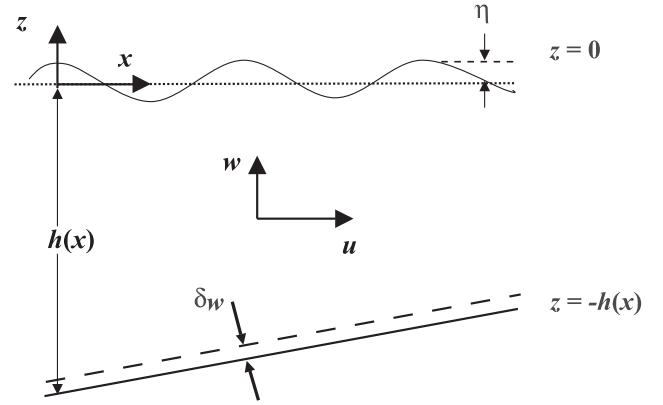
Figure 1. Definition sketch of variables and coordinate system for waves propagating over a planar, sloping seabed.
