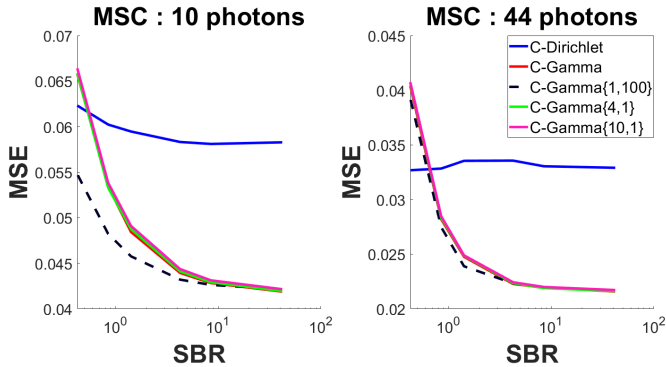
Fig. 2. MSE of \mathbf{R} obtained with the different competing methods as function of the SBR. The left (resp. right) subplot corresponds to MSC equals to 10 (resp. 44) photons.
