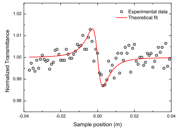
Fig. 1. Divided closed-aperture Z-scan trace for the SLG taken at a pulse energy of 100 nJ, corresponding to an irradiance of 8.14 GW cm -2 . The theoretical fit (red line) was calculated using a \tilde{n}(I) coefficient of -6.8 \times 10^{-9} cm 2 W -1 .
