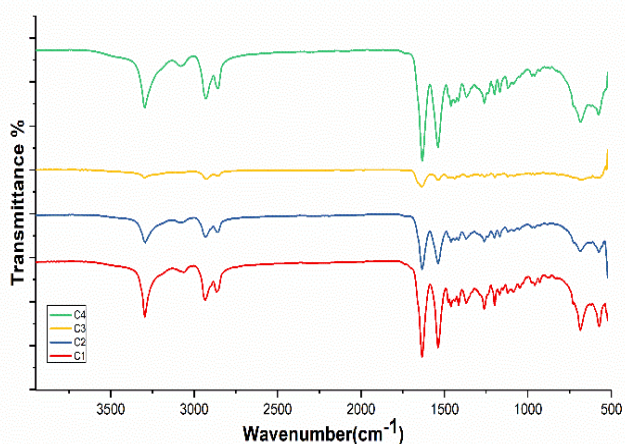
Fig. 4. FTIR plots of the variable concentration samples.
