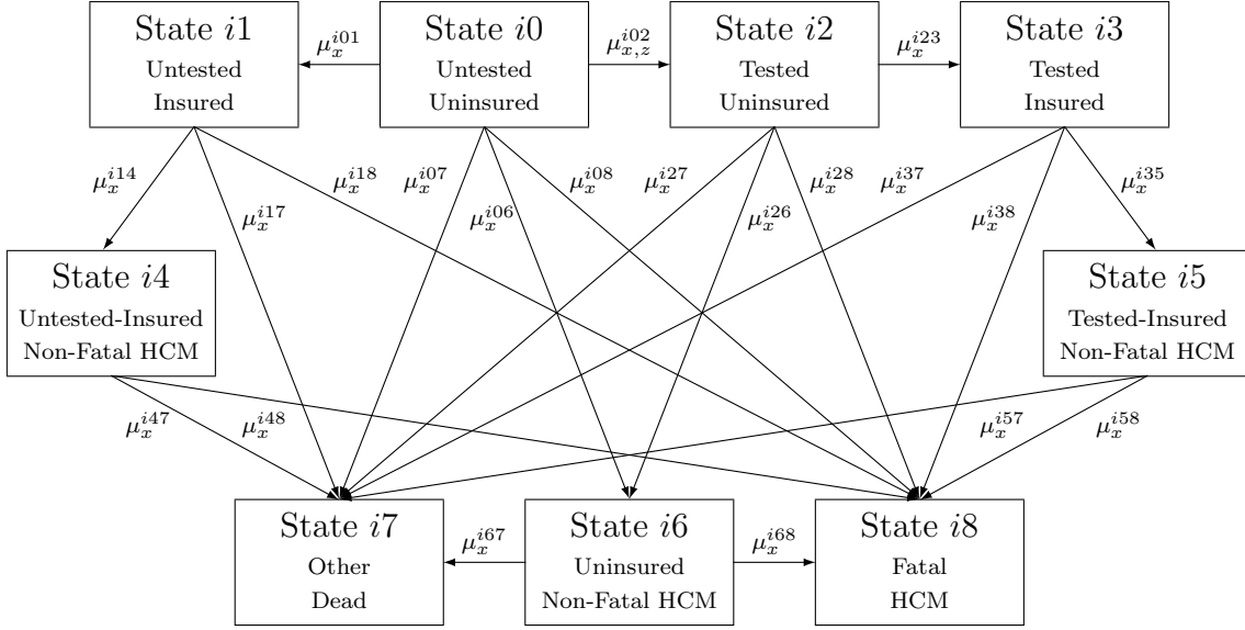
Figure 1: A mathematical model of the life history of a person in the i th of several sub-populations defined by HCM genotype. The life history includes biological events and decisions made by the individual. In \mu_{x,z}^{i02} , z refers to duration in state i0 since (if) a proband appeared in the family.
