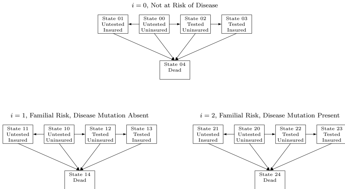
Figure 3: A mathematical model of uptake of genetic testing and purchase of life insurance for a population in which one sub-population ( i = 2 ) carries a mutation associated with a dominantly inherited genetic disease.
