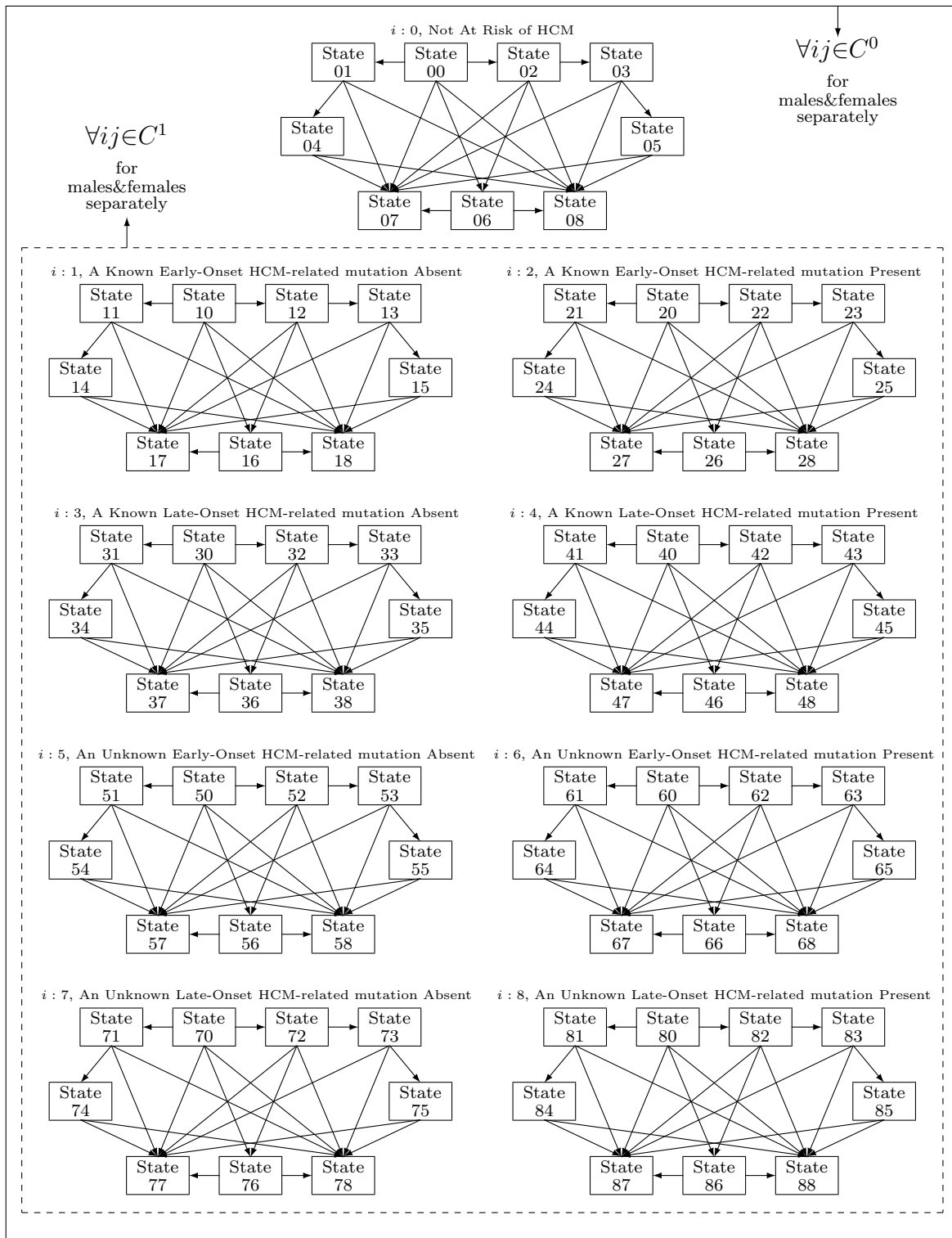
Figure 2: A mathematical model of the life history of a randomly chosen individual, present in one of the states i0 at birth with probabilities determined by HCM-related mutation prevalences and Mendel's laws. See Section 4.5, and Appendix A.
