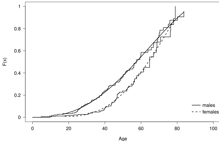
Figure 4: Late-Onset Penetrance Rate of HCM from Christiaans et al. (2011)
