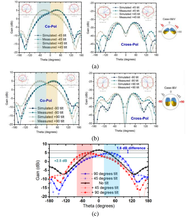
Fig. 10. Simulated and measured E-plane (YOZ-plane) radiation pattern of the proposed antenna under (a) \pm 45^\circ tilt. (b) \pm 90^\circ tilt. (c) Simulated E-plane radiation patterns for \pm 45^\circ and \pm 90^\circ physical tilts of the antenna.
