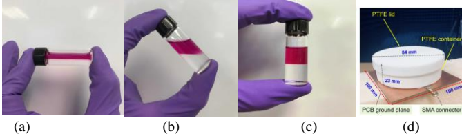
Fig. 5. (a) Illustration of the two liquid layers under a flat-ground case (Case-III). (b) 45° tilt (Case-II and Case-IV). (c) 90° tilt (Case-I and Case-V). Potassium permanganate ( \text{KMnO}_4 , 3 mg) was added to the low-density top layer to aid visualisation. (d) Picture of the fabricated antenna prototype. The overall dimensions of the antenna prototype are shown as well.
