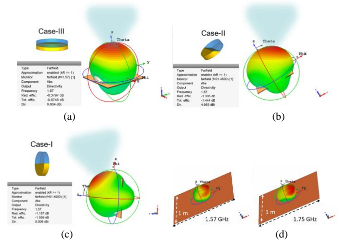
Fig. 8. 3D radiation patterns and gains of the proposed antenna at 1.57 GHz under three different cases of tilt. (a) Flat. (b) 45^\circ tilt. (c) 90^\circ tilt. (d) Radiation patterns at 1.57 and 1.75 GHz when the antenna is mounted on a large metal ground of 1 m \times 1 m.
