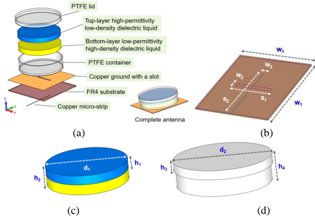
Fig. 1. (a) Materials and overall assembly of the proposed liquid antenna. Detailed dimensions of (b) the PCB (FR4 substrate \epsilon_r = 4.5 , thickness = 1.6 mm). (c) Two layers of liquid resonators. (d) Liquid container and lid (made of PTFE, \epsilon_r = 2.1 , thickness = 2 mm). The size of the PCB is w_1 \times w_1 = 100 \times 100 \text{ mm}^2 , s_2 = 65 \text{ mm} , w_3 = 1 \text{ mm} , s_1 = 44 \text{ mm} , w_2 = 3 \text{ mm} , d_1 = 79 \text{ mm} , h_2 = 19 \text{ mm} , h_1 = 9.5 \text{ mm} , d_2 = 84 \text{ mm} , h_4 = 23 \text{ mm} and h_3 = 8 \text{ mm} .
