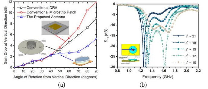
Fig. 11. (a) Comparison of antenna gain drop at the vertical direction during rotation for three different antennas including the proposed antenna and conventional DRA and patch. (b) Tunable resonances of the antenna by using liquids with different relative permittivities in accordance to Fig. 4. An example of crossed slot for CP radiation is given.
