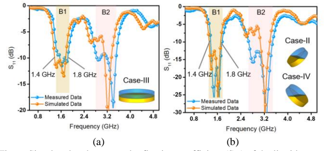
Fig. 6. Simulated and measured reflection coefficient ( S_{11} ) of the liquid antenna under (a) Case-III (antenna is parallel to flat ground). (b) Case-IV (antenna is tilted 45^\circ ).
