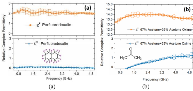
Fig. 3. Measured frequency dependence of the relative complex permittivity of (a) perfluorodecalin (PFD). (b) 67 wt. % acetone / 33wt. % acetone oxime mixture. Standard derivation error bars are given.
