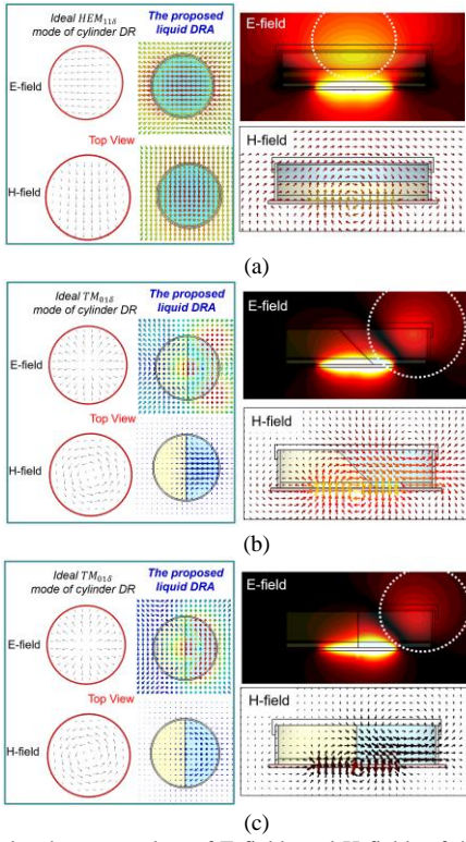
Fig. 9. Simulated contour plots of E-fields and H-fields of the antenna under the three aforementioned cases. (a) Case-III. (b) Case-II and Case-IV. (c) Case-I and Case-V. The field distributions of the ideal TM_{01\delta}^z and HEM_{11\delta} modes for cylinder DR are presented for comparison (taken from [18]).
