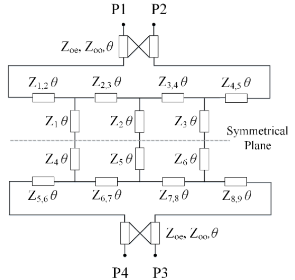
Fig.1. Topology of the proposed wideband BPFs.
