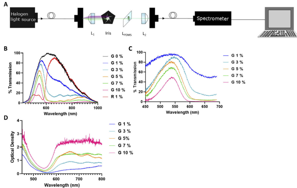
Fig. 3. The IFLs have the ability to filter light in the visible spectrum. Transmission schematic (A) for setup with fibre coupled white light source into a collimating lens ( L_1 ), iris and PDMS filtering lens ( L_{PDMS} ). There is an additional lens to focus the light into a second optical fibre ( L_2 ) feeding to the fibre coupled spectrometer. (B) % transmission spectra measured by the spectrometer for the green IFLs (labelled G) and red 1% IFLs (labelled R) over the visible spectrum. (C) Transmission spectra for green IFLs 1% to 10%. The green IFLs show a concentration dependent response with 10% lens blocking more light than the 1% IFLs across the spectrum. Transmission peak at 545 nm displaying the IFLs ability to transmit green light. (D) Optical density plot for the filtering lens showing that the higher doped IFLs had a greater optical density than the lower doped IFLs.
