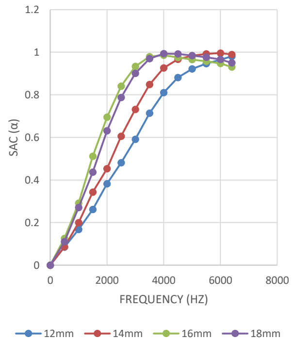
Fig. 1 Sound Absorption Coefficient versus Frequency of LDF for thickness of 12 mm, 14 mm, 16 mm and 18 mm with density of 120 kg/m 3 at frequency range of 0 Hz - 6400 Hz
