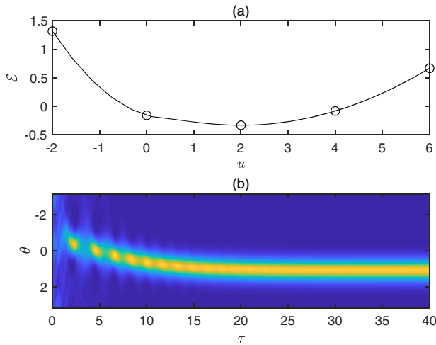
FIG. 3. (a) Numerically calculated scaled energy \mathcal{E} versus the scaled velocity u for a = 1.5 and g = -2 , showing an energy minimum for u = 2 . The circles provide the approximate energy in Eq. (21) for the allowed quantized values of the velocity u = 0, \pm 2, \dots (b) Color coded plot of the time evolution of the probability density |\varphi(\theta, \tau)|^2 for \Lambda = -0.05 , and starting from a random initial condition.
