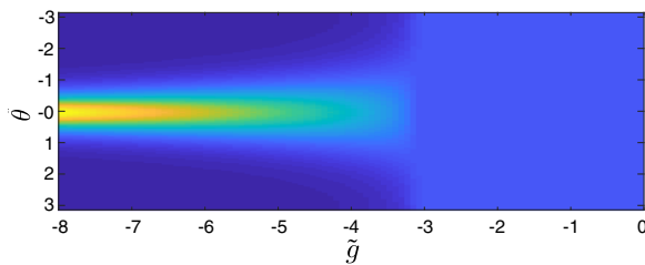
FIG. 2. Color coded plot of the chiral soliton density profile |\chi(\theta)|^2 obtained from the numerical solutions versus the angular variable \theta and \tilde{g} .
