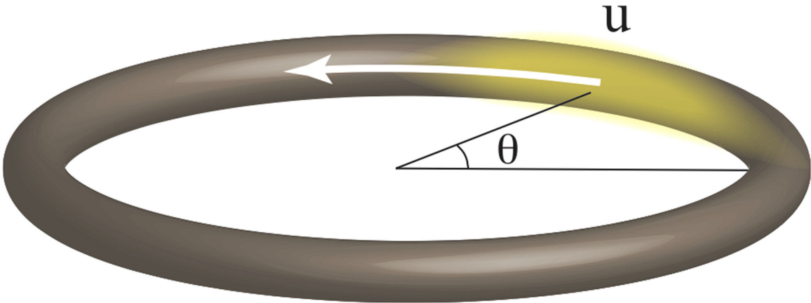
FIG. 1. The tightly confined ring with radius R circumferentially traps the Bose-Einstein condensate such that the dynamics is effectively one-dimensional along the azimuthal or \theta direction. The chiral soliton of velocity u , indicated by the yellow region, is only allowed to travel in one specific direction given by the parameters of the current nonlinearity.
