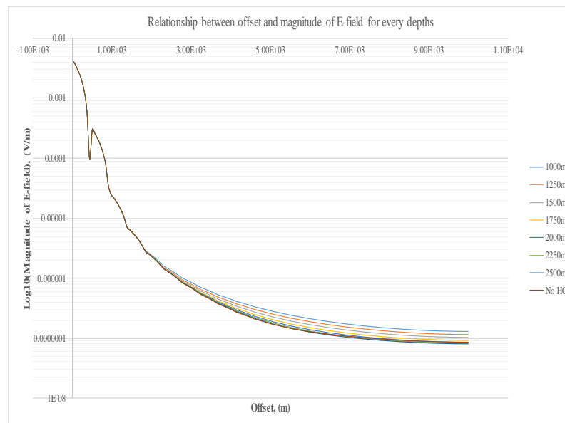
Figure 3. Offset against log10 of magnitude of E-field for each hydrocarbon (HC) depth.
