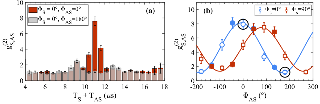
FIG. 3. (a) Examples of g_{S,AS}^{(2)} between Stokes and anti-Stokes photons when an AFC with \tau_{\text{IFC}} = 2 \mu\text{s} is prepared in both the Stokes and the anti-Stokes mode in the IFC. The cases of constructive (darker bars) and destructive (lighter bars) interference are shown. For both measurements, the integration time is 10 h, approximately. (b) Interference fringes measured by tuning the frequency of the anti-Stokes filter AFC (i.e., by tuning \Phi_{AS} ) in two different bases, selected by changing the frequency of the filter AFC for the Stokes photon. The circled points are the ones related to Fig. 3(a). The filled points are those used to calculate the S parameter (integration time 6.5 h per point). The remaining data point are the result of 5.5 h of integration each.
