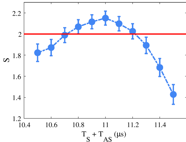
FIG. 4. Bell inequality S parameter measured as a function of T_S + T_{AS} . The red line denotes the threshold S = 2 for violating the CHSH inequality.
