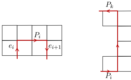
Figure 2: Two impossible configurations.
