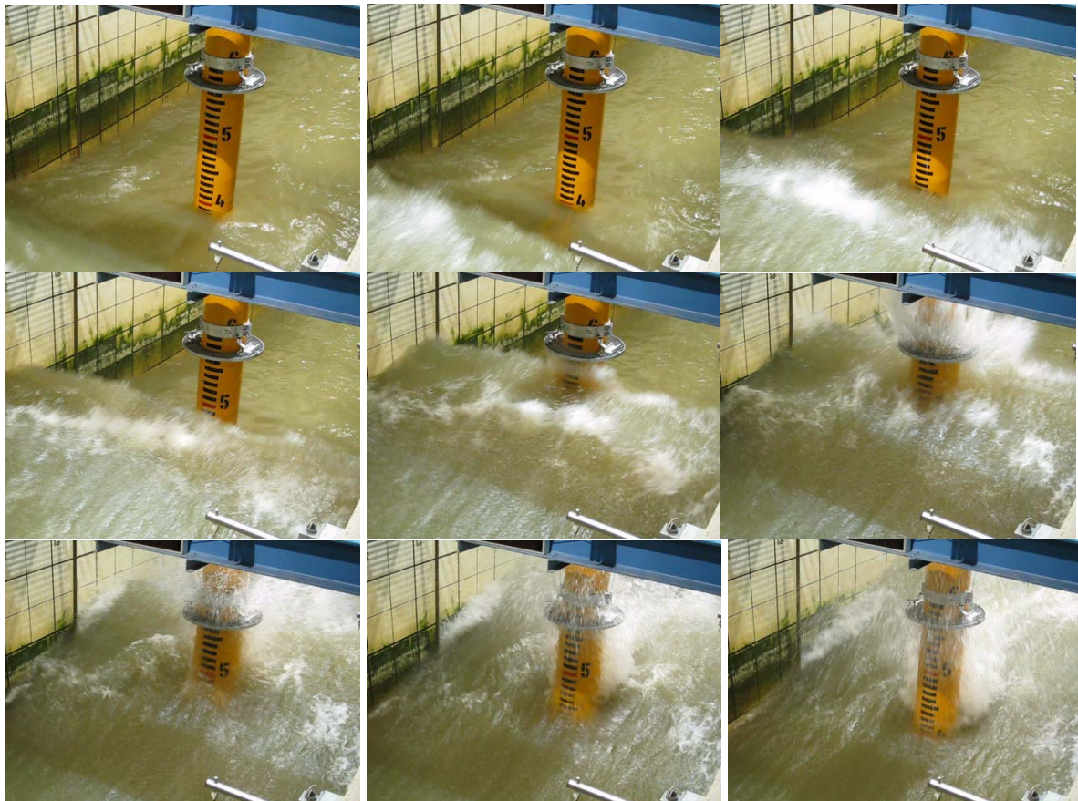
Fig. 2: Pictures ( \Delta t = 0.20 s) of impacting irregular wave on grate platform (porosity 80%) at level +1.75. Maximum load 0.51 kN for h = 3 m, H_{m0} = 1.0 m and T_p = 5.9 s, all values in model scale.
