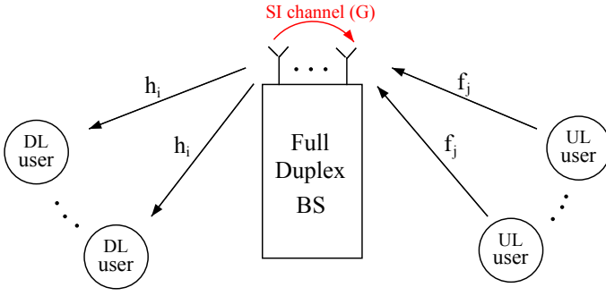
Fig. 1. System model with a FD radio BS with N antennas, K HD downlink users and J HD uplink users.
