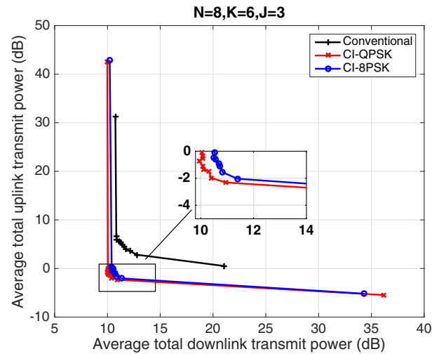
Fig. 6. Average system object trade-off region achieved by the proposed scheme versus the conventional scheme \Gamma^{UL} = 0\text{dB} and \Gamma^{DL} = 10\text{dB}
