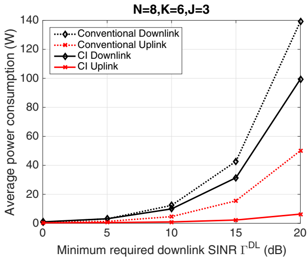
Fig. 3. Average power consumption versus minimum required downlink SINR when \lambda_1 = 0.9, \lambda_2 = 0.1 and \Gamma^{UL} = 0\text{dB} for QPSK modulation
