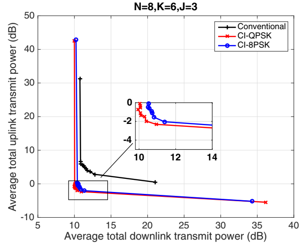
Fig. 6. Average system object trade-off region achieved by the proposed scheme versus the conventional scheme \Gamma^{UL} = 0\text{dB} and \Gamma^{DL} = 10\text{dB}
