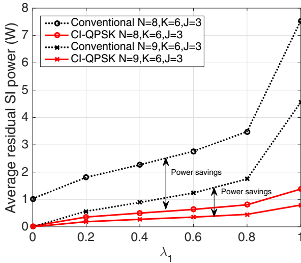
Fig. 4. Average residual SI power versus \lambda_1 when \Gamma^{UL} = 5\text{dB} and \Gamma^{DL} = 10\text{dB}
