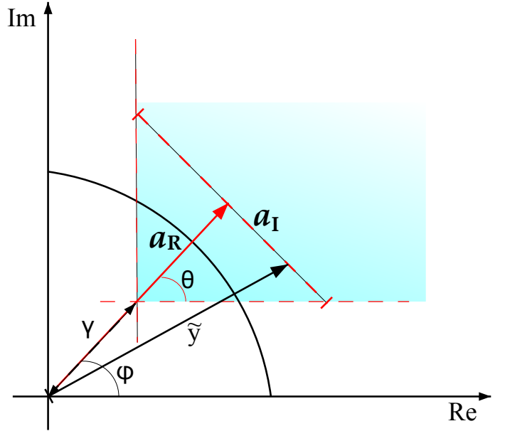
Fig. 2. Constructive interference region for a QPSK constellation point
