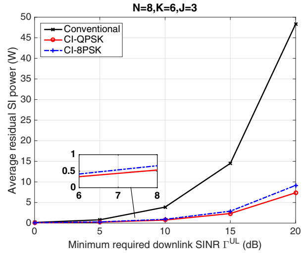
Fig. 5. Average residual SI power versus minimum required downlink SINR when \lambda_1 = 0.9, \lambda_2 = 0.1 and \Gamma^{UL} = 5\text{dB}
