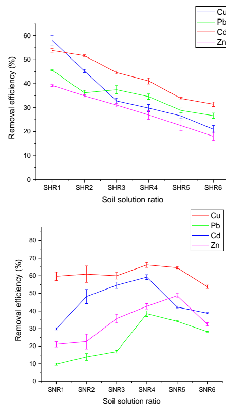
Fig 3. Effect of soil-solution ratio of SN and SH on the removal of heavy metals from soils (time = 6 hr concentration = 3). Each point is the average of triplicate samples. Soil: shikakai solution (w/v) - SHR1= 1.2%; SHR2= 1.3%; SHR3= 1.4%; SHR4= 1.5%; SHR6= 1.6%; Soil : soapnut solution (w/v) - SNR1= 1.2%; SNR2= 1.3%; SNR3= 1.4%; SNR4= 1.5%; SNR6= 1.6%.
