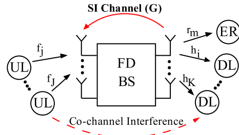
Fig. 1. A multi-user FD SWIPT system.
