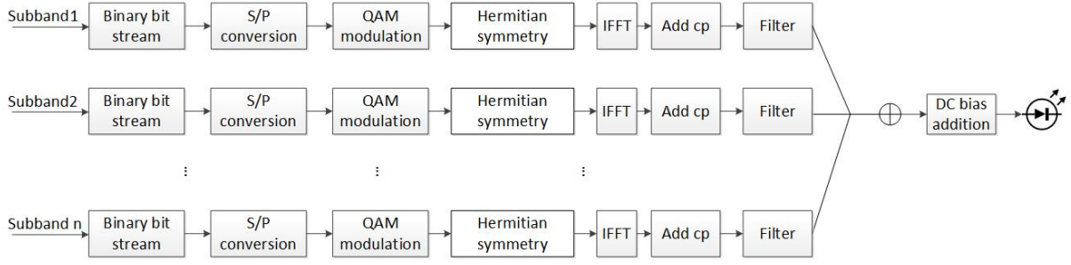
Fig. 1. Transmitter of the VLC F-OFDM system.
