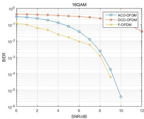
(b) BER of three OFDM schemes for 16QAM
