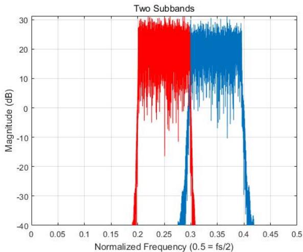
Fig. 5. Signals of two subbands.
