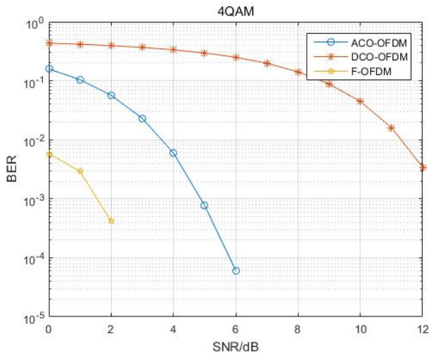
(a) BER of three OFDM schemes for 4QAM
