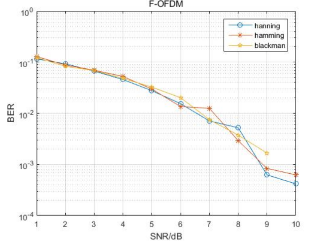
Fig. 4. BER of different windows.
