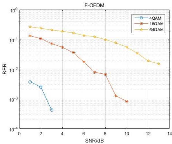
Fig. 6. BER vs. SNR for different QAM schemes in the F-OFDM VLC system.
