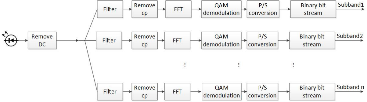
Fig. 2. Receiver of the VLC F-OFDM system.
