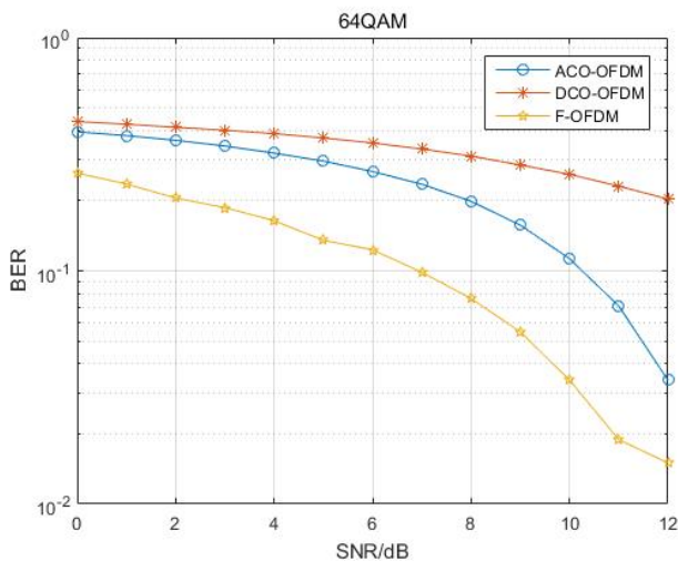
(c) BER of three OFDM schemes for 64QAM
