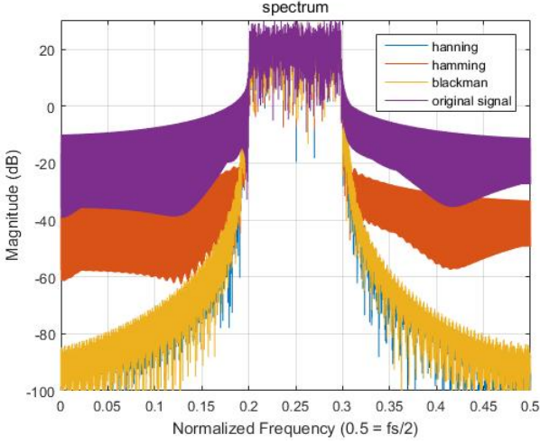
Fig. 3. Signals with different windows.
