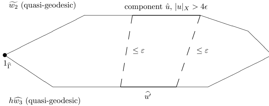
Figure 1: The paths \tilde{w}_2 and h\widehat{w}_3 in \hat{\Gamma} : bounded coset penetration
