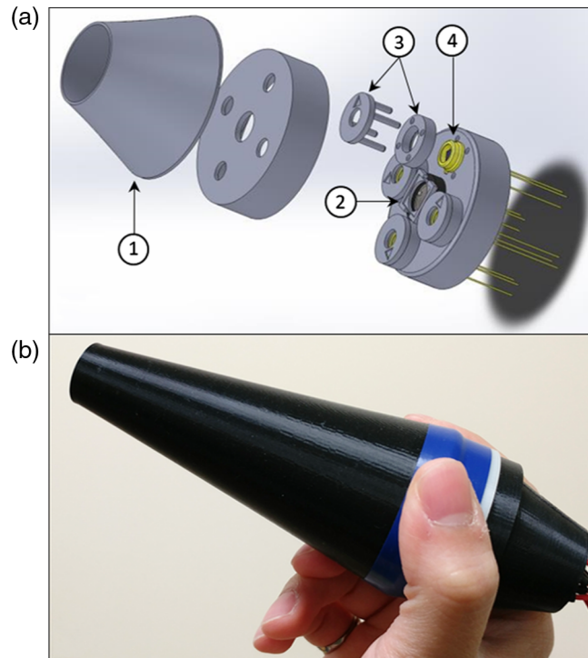
Fig. 1 (a) Illustration of the Stokes polarimetry probe head components, including (1) conical front piece, (2) laser diode and collimator, (3) parts to hold polarizing film, and (4) photodiodes. (b) Photo of the probe in hand.
