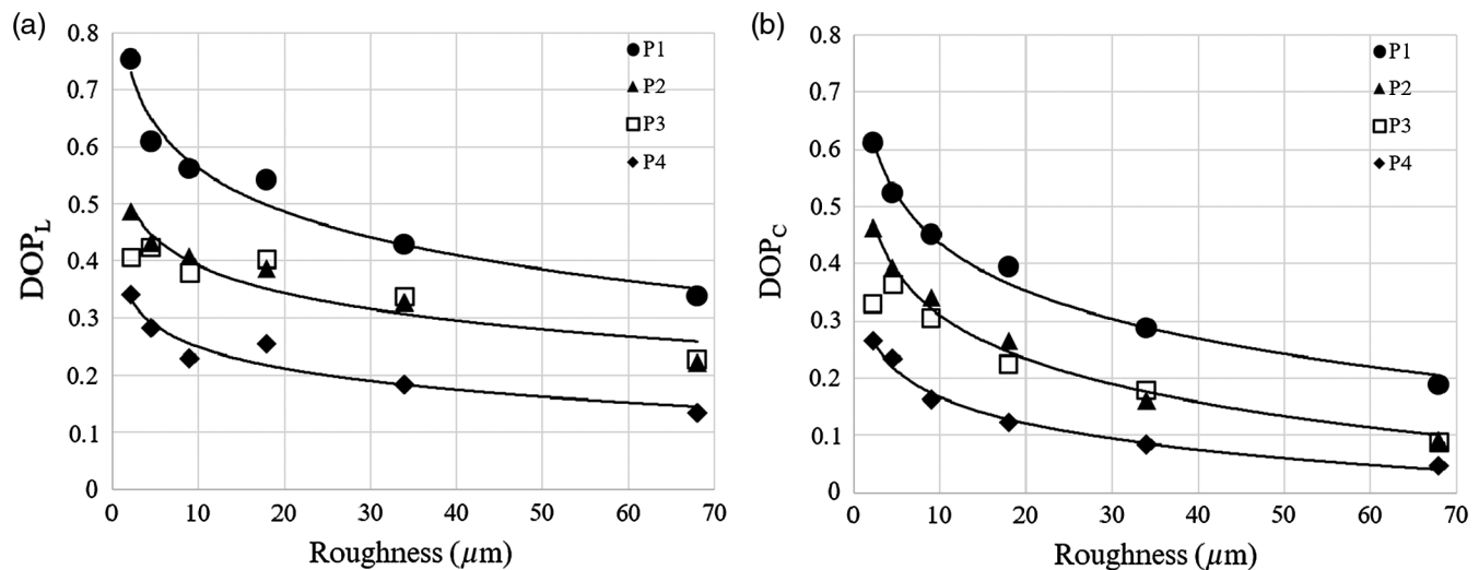
Fig. 2 DOP versus phantom roughness with trend lines for (a) linear and (b) circular input polarizations. Trend lines shown for P1, P2, and P4.
