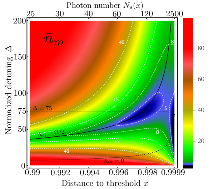
FIG. 2. Steady-state phonon number as a function of \Delta and x , as obtained from a semiclassical description of the DOPO and a thermal phonon number \bar{n}_{\text{th}} = 100 (achievable either with cryogenics [41] or via a standard sideband precooling stage). We choose typical parameters for cWGM resonators [10]: \Omega = 10 , \eta_{\text{OM}} = 10^{-4} , and Q = 10^6 . Note that typical optical decay rates are in the megahertz range, although only normalized quantities are relevant for our results. The signal steady-state photon numbers \bar{N}_s(x) corresponding to the ticked x values are shown on the upper axis, showing that cooling is effective even with just \sim 100 photons. On the other hand, c-MoP theory has allowed us to prove that the cooling region closer to the threshold disappears once this more accurate approach is used (see Fig. 3).
