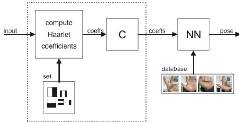
FIG. 5: Structure of the classifier illustrating the transformation \mathbf{T} (dotted box), approximated using Haarlets. The Haarlet coefficients are computed on the input sample. The approximated coefficients (that would result from \mathbf{T} ) are computed as a linear combination \mathbf{C} of the Haarlet coefficients.
