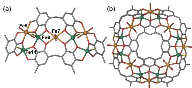
Figure 2. Arrangement of Fe II and Fe III ions on the framework of 1 . (a) Two [Fe 3 O 3 ] units connected through a bridging Fe II ion (Fe7), and (b) arrangement of Fe II ions along the metal-organic hemispheres. PgC 6 alkyl chains and H atoms omitted for clarity. Color code: Fe II – orange, Fe III – green, Cl – yellow, O – red, C – gray.
