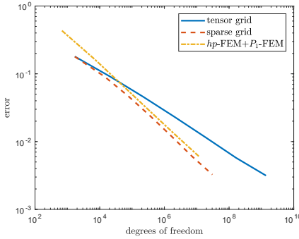
FIG. 8.3. Convergence of the error in the energy norm versus the number of degrees of freedom of the extended problem with the right-hand side f \equiv 1 and s = 3/4 . P_1 -FEM on corner-refined, regular simplicial meshes is used in \Omega . We compare hp -FEM in (0, \mathcal{Y}) with tensor grid and sparse grids, the latter two employing radical meshes in (0, \mathcal{Y}) .
