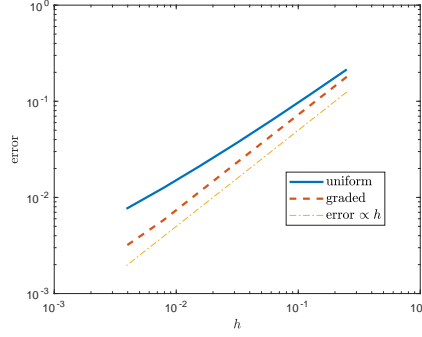
FIG. 8.2. Convergence of the error in the energy norm versus meshwidth in \Omega with the right-hand side f \equiv 1 and s = 3/4 , leading to a solution with singular behavior near the re-entrant corner (0, 0) . Error graphs are shown for a P_1 -FEM on uniformly refined meshes in \Omega and on meshes refined towards the corner.
