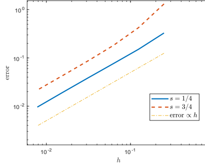
FIG. 8.4. Convergence of the error in the energy norm versus the meshwidth in \Omega with the (smooth) exact solution given by (8.1) for two different values of s . A P_1 -FEM on uniformly refined meshes in \Omega and hp -FEM in (0, \mathcal{Y}) is used.
