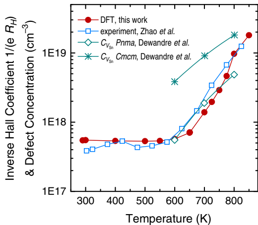
FIG. 7. Inverse Hall coefficients, 1/(eR_H) , and Sn vacancy concentrations, C_{V_{Sn}} , in SnSe as a function of temperature. Red solid circles show the average inverse Hall coefficient obtained here from Boltzmann transport calculations assuming hole-doping concentration of n_p = 5 \times 10^{17} \text{ cm}^{-3} at ambient temperature and the adjusted band gaps from Fig. 4(c). Blue open squares show the corresponding experimental data by Zhao et al. [1]. Cyan diamonds and stars show the carrier concentration obtained from the \text{Sn}^{2-} vacancy model by Dewandre et al. [13] for the Pnma and Cmcm/Bmmm phases, respectively.
