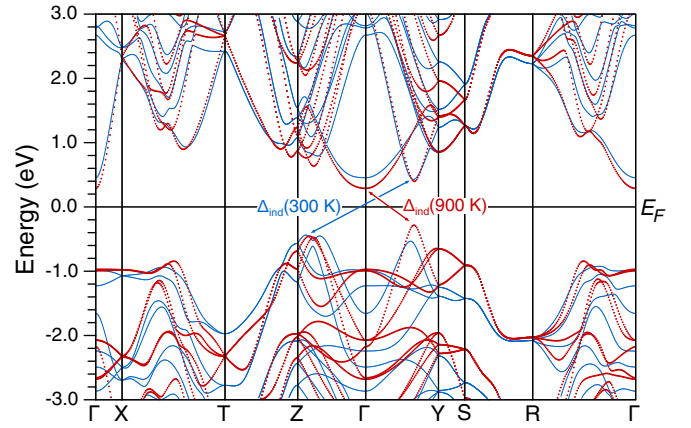
FIG. 3. Calculated band structure of SnSe at 300 K (solid lines, blue) and 900 K (dotted lines, red). The special points refer to the Pnma Brillouin zone, which was used for both calculations to allow for a direct comparison.
