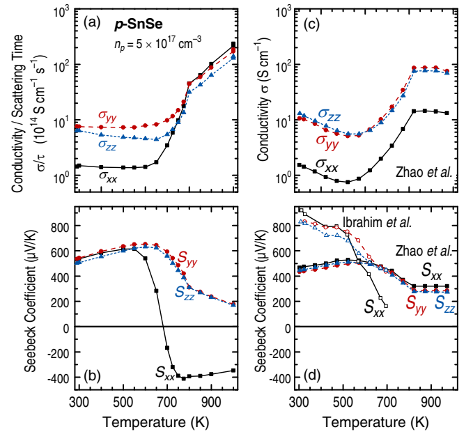
FIG. 6. (a) Calculated electrical conductivity \sigma divided by the scattering time \tau of p -SnSe and (b) calculated Seebeck coefficient as a function of temperature. A hole-doping concentration of n_p = 5 \times 10^{17} \text{ cm}^{-3} at ambient temperature and the adjusted band gaps from Fig. 4(c) were used in both cases. (c, d) Corresponding experimental results by Zhao et al. [1] (solid symbols) and Ibrahim et al. [36] (open symbols).
