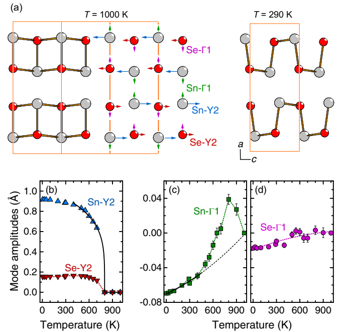
FIG. 2. (a) Atomic displacement patterns of the active symmetry-adapted distortion modes of SnSe. The arrows are not to scale. (b–d) Amplitudes of the distortion modes as a function of temperature, see text for details. Solid black lines in (b,c) are fits to the data as explained in the text, the dashed line in (c) shows a quadratic extrapolation of the 4–400-K data, and the dotted lines in (b–d) are guides to the eye.
