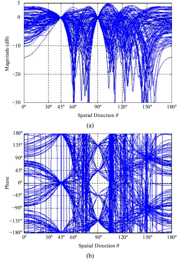
Fig. 1. Far-field radiation (a) magnitude and (b) phase patterns for 100 random transmission states in the synthesized dual-beam BPSK-QPSK dynamic DM system. PE_{DM} = 33\% .
