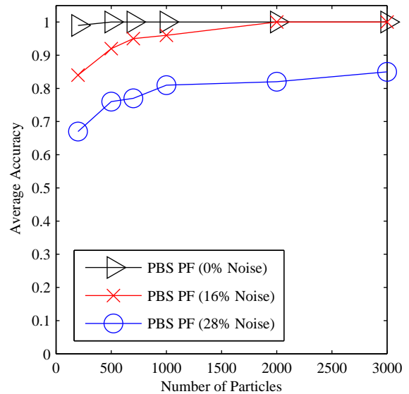
Figure 8: The average accuracy of the PBS Particle Filter with different numbers of particles
